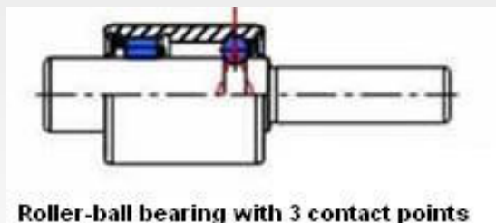
Roller-ball bearing with 3 contact points
