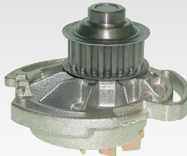
Pulley 18 teeth
